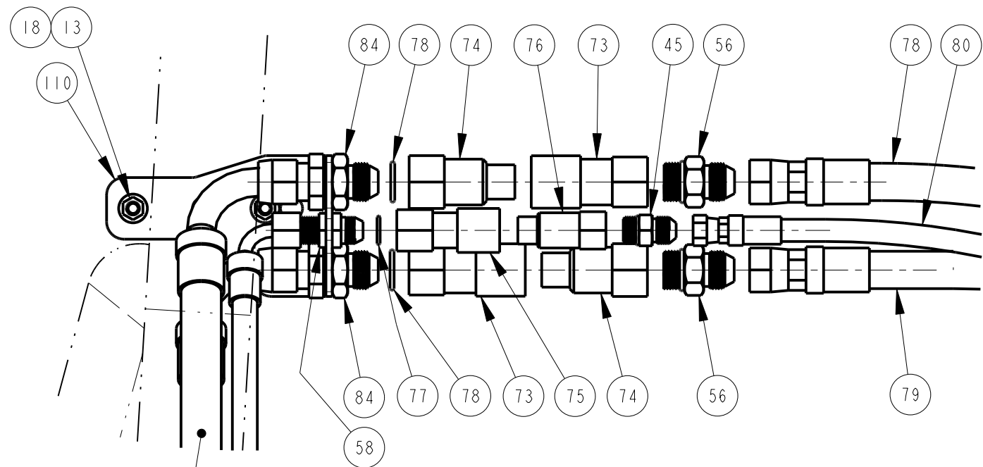
VIEW V (SHEET 9)
