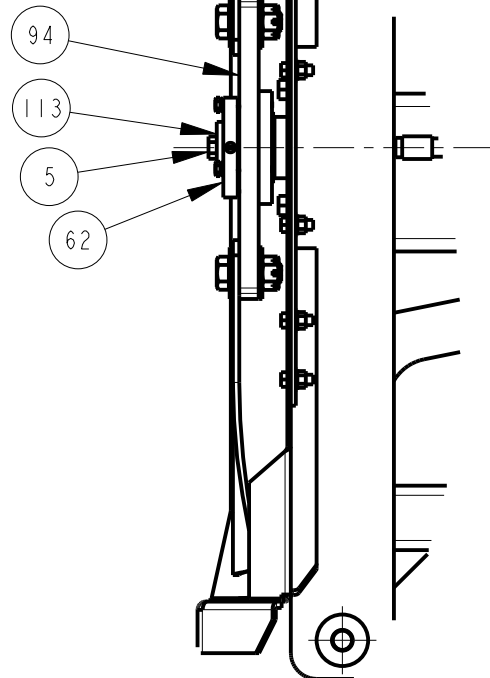
DETAIL P (SHEET 8)
