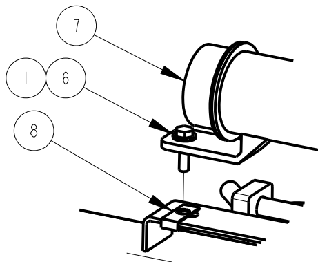
CANISTER MOUNTING (CAP NOT SHOWN)
