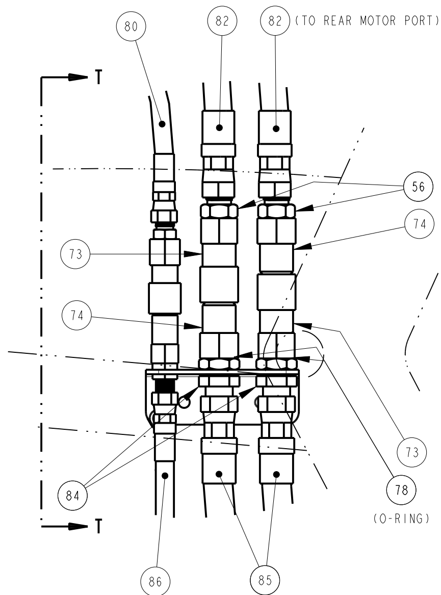
DETAIL R (SHEET 9)
