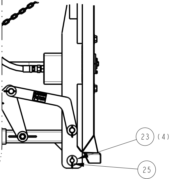
REAR COMPONENTS DETAIL (2 PUMP HOSES NOT SHOWN)
