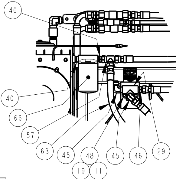
REAR COMPONENTS DETAIL (2 PUMP HOSES NOT SHOWN)
