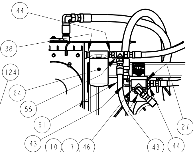
REAR COMPONENTS DETAIL
