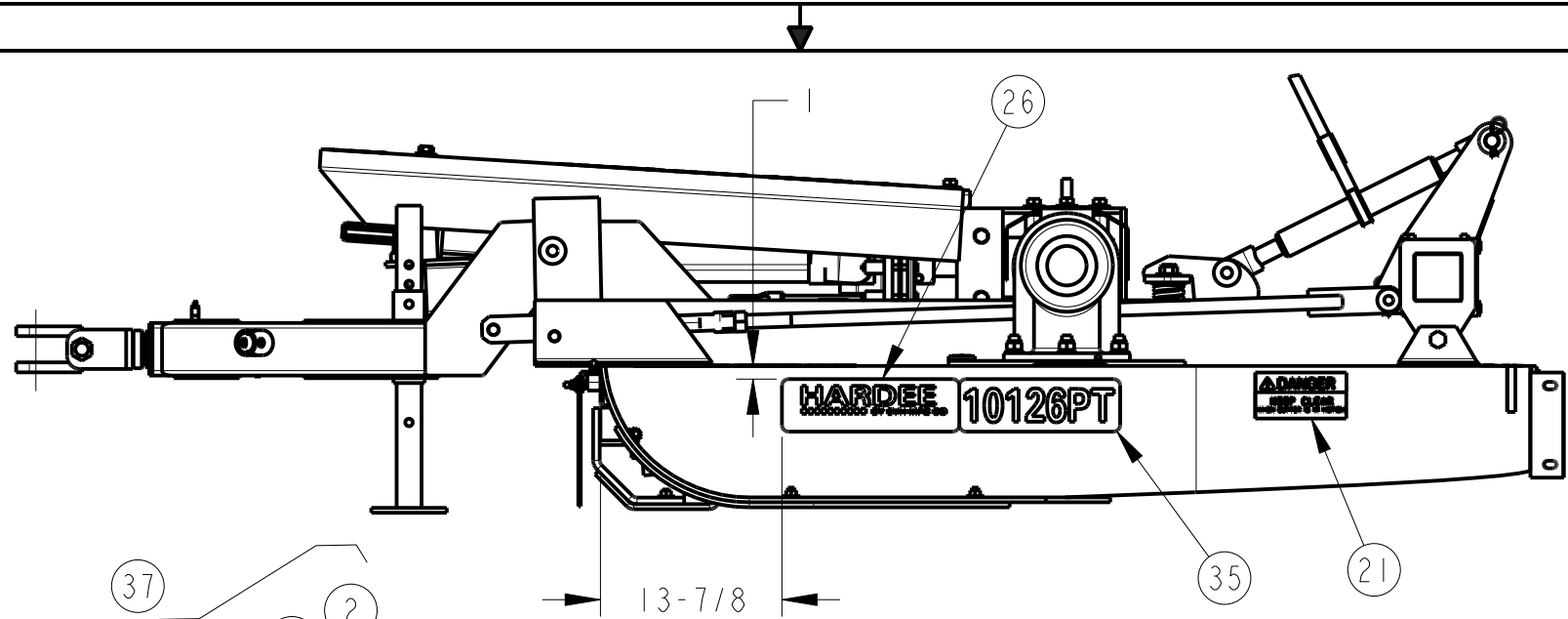
DECK LEFT VIEW (TAILWHEEL ARMS NOT SHOWN)
