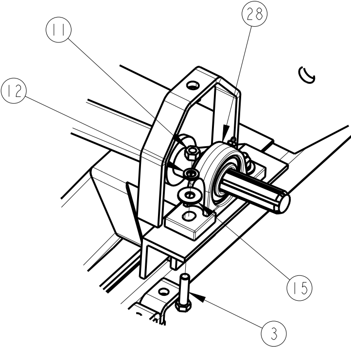
DETAIL A
